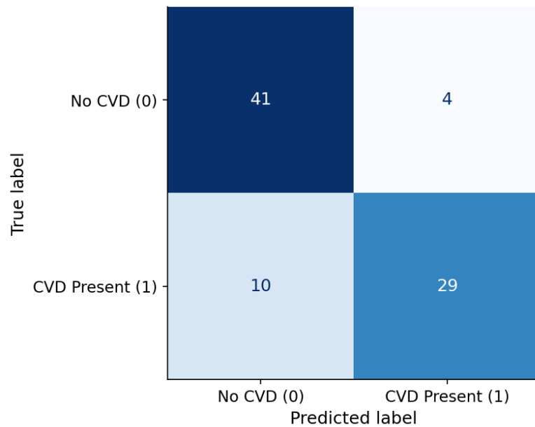
Figure 10: Logistic Regression Confusion Matrix Test Set Results
